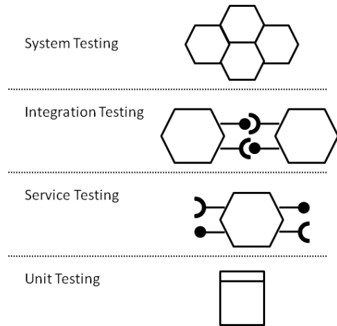
Figure 1. SOA testing layers as presented in [18]
