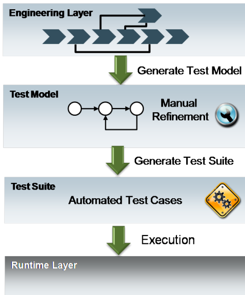
Figure 3. Envisioned testing process
