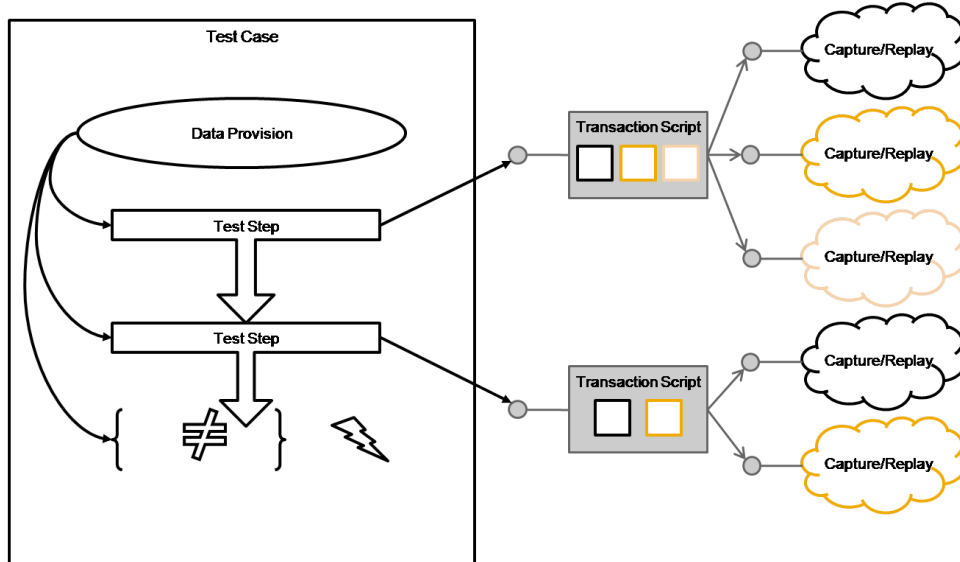
Figure 2. Industrial reuse concept of capture/replay scripts
